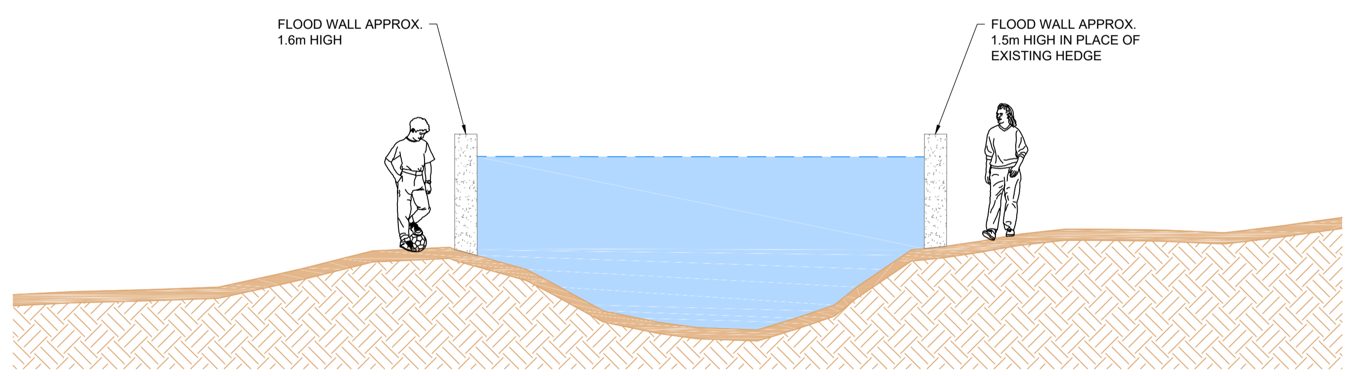
SECTION A-A: FLOOD DEFENCE WALLS 1:50
